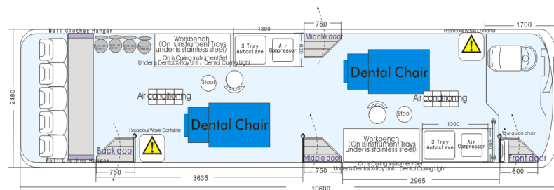
Potential Design Layout of the MDC
